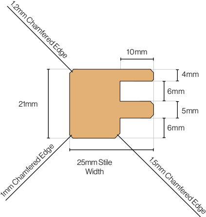
Brooklyn Oak Stile Cross Section
