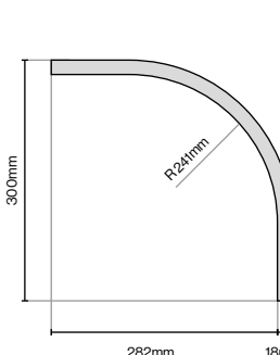
Curved Torus Plinth 300mm (L) x 300mm (W) x 150mm (H)
