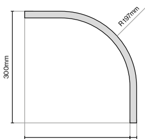
Curved Tangent Pelmet 300mm (L) x 300mm (W) x 150mm (H)
