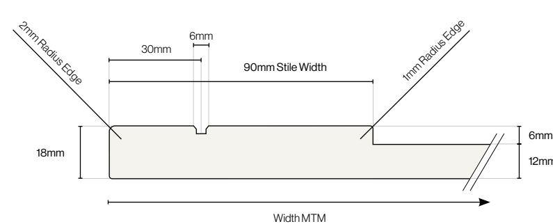
Wellington Stile Cross Section
