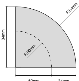
Classic Cornice Quadrant 84mm (L) x 84mm (W) x 63mm (H)
