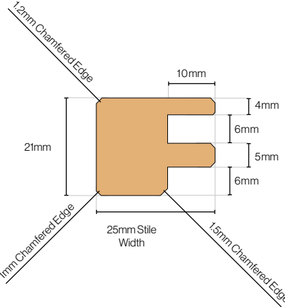
Brooklyn Oak Stile Cross Section
