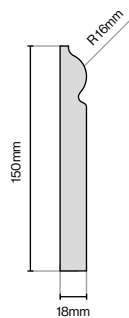
Torus Plinth 3050mm Lengths
