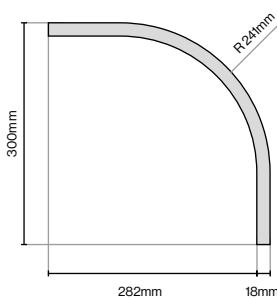
Curved Tangent Pelmet 300mm (L) x 300mm (W) x 150mm (H)
