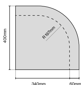
Curved Tangent Cornice 400mm (L) x 400mm (W) x 44mm (H)
