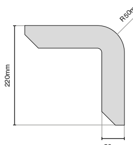
Modern Cornice / Pelmet Quadrant 220mm (L) x 220mm (W) x 30mm (H)
