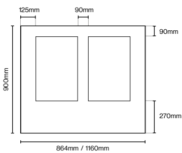
Double Feature Panel 900mm (H) x 864mm (W) / 900mm (H) x 1160mm (W) EXS PTO Not available Primed. Standard Sizes Only.
