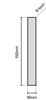
Plain Plinth 3050mm Lengths
