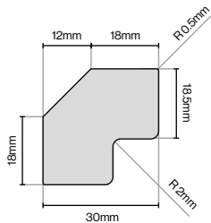
Corner Post 3050mm Lengths
