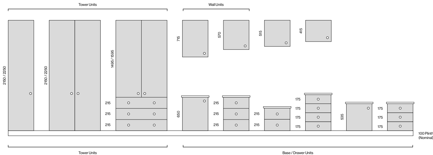
Standard Bedroom / 2150mm / 2250mm / Base and Full Height Unit Door Configurations
