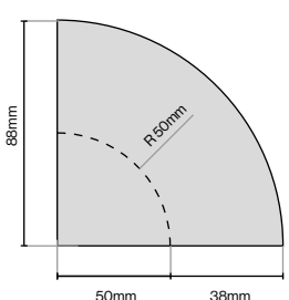
Tangent Cornice Quadrant 88mm (L) x 88mm (W) x 44mm (H)
