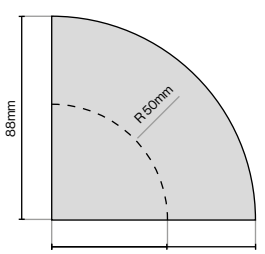
Tangent Cornice Quadrant 88mm (L) x 88mm (W) x 44mm (H)
