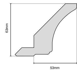
Classic Cornice 3050mm Lengths
