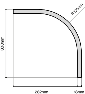
Curved Plain Plinth 300mm (L) x 300mm (W) x 150mm (H)
