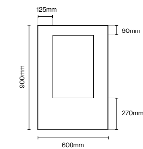
Single Feature Panel 900mm (H) x 600mm (W) EXS PTO Not available Primed. Standard Sizes Only.
