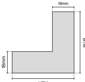
MTM Corner Post 715mm (150 x 150mm Max)
