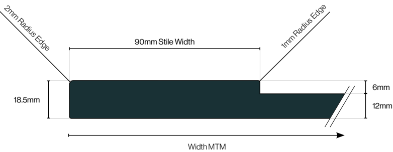
Hartford Stile Cross Section
