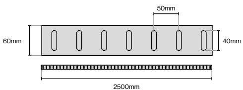
Fluted Rail 2500mm Lengths
