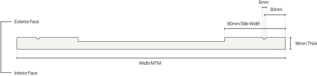
Wellington Door Cross Section
