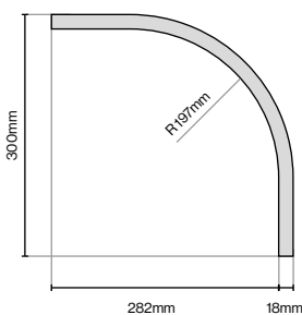
Curved Torus Plinth 300mm (L) x 300mm (W) x 150mm (H)
