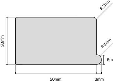
Under Cornice (Smooth) 3050mm Lengths
