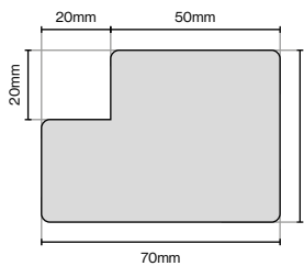
Square Pilaster 3050mm Lengths
