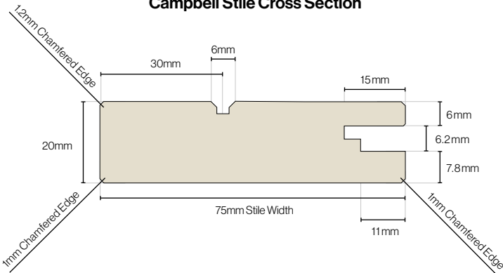
Campbell Stile Cross Section
