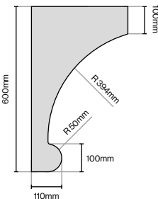
French Mantle Corbel 350mm (L) x 90mm (H) x 600mm (H)
