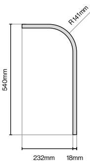
Curved Plain Plinth 540mm (L) x 250mm (W) x 150mm (H)
