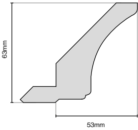
Classic Cornice 3050mm Lengths
