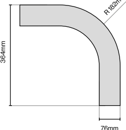
Curved Classic Cornice (Grained) 364mm (L) x 364mm (W) x 63mm (H)
