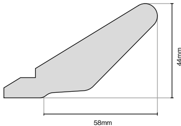
Tangent Cornice 3050mm (L) x 72mm (W) x 44mm (H)
