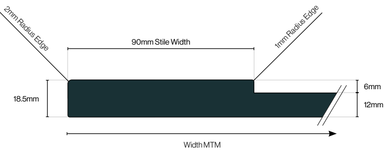
Hartford Stile Cross Section
