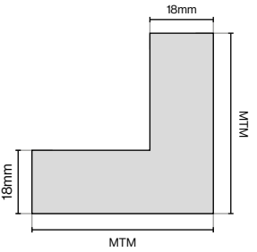
MTM Corner Post 715mm (150 x 150mm Max)
