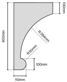
French Mantle Corbel 350mm (L) x 90mm (H) x 600mm (H)
