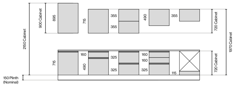
1970mm / 2150mm / Base and Wall Unit Door Configurations
