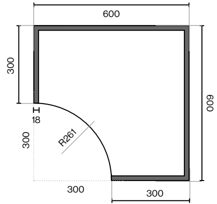
300mm Concave Door 300mm x 300mm Concave Door for 600mm Wall Unit
