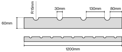
Wine Rack Rail 1200mm (L) x 18mm (W) x 60mm (H)
