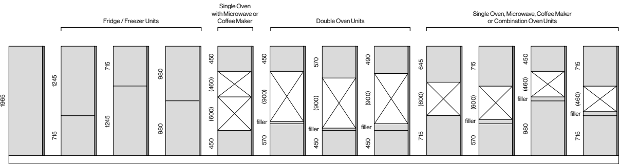
1970mm / Full Height Unit Door and Appliance Configurations
