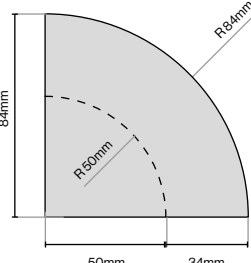
Classic Cornice Quadrant 84mm (L) x 84mm (W) x 63mm (H)
