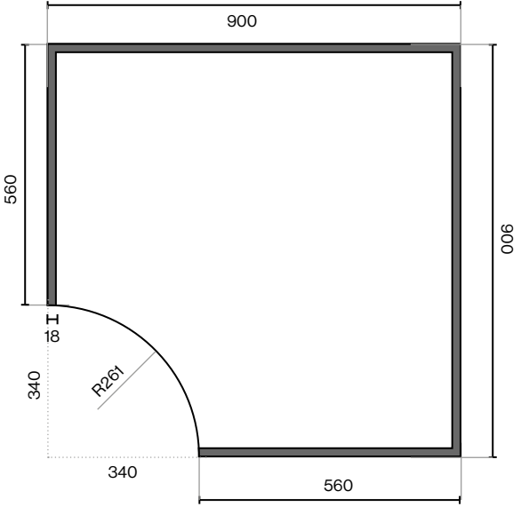
340mm Concave Door 340mm x 340mm Concave Door for 900mm Base Unit
