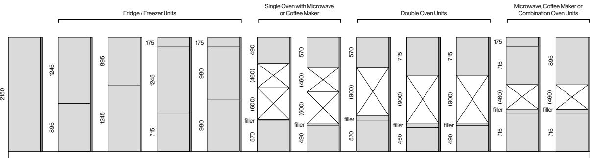
2150mm / Full Height Unit Door and Appliance Configurations
