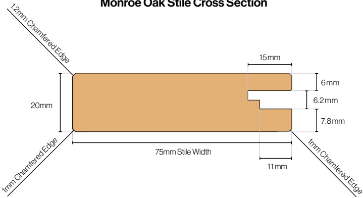
Monroe Oak Stile Cross Section
