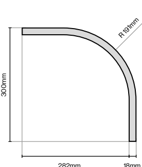
Curved Plain Plinth 300mm (L) x 300mm (W) x 150mm (H)
