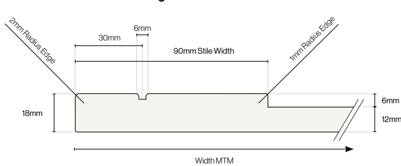
Wellington Stile Cross Section
