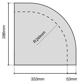
Curved Classic Cornice 386mm (L) x 386mm (W) x 63mm (H)
