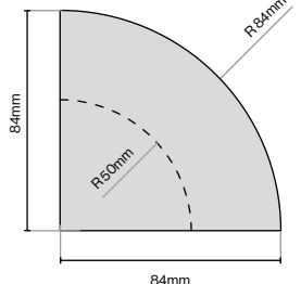
Classic Cornice Quadrant (Grained) 84mm (L) x 84mm (W) x 63mm (H)
