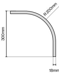
Curved Torus Plinth (Smooth) 300mm (L) x 300mm (W) x 150mm (H)
