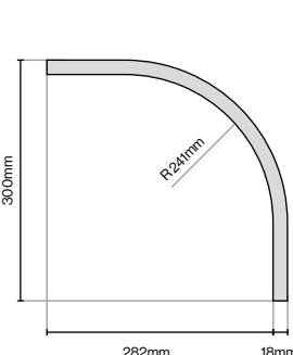
Curved Torus Plinth 300mm (L) x 300mm (W) x 150mm (H)
