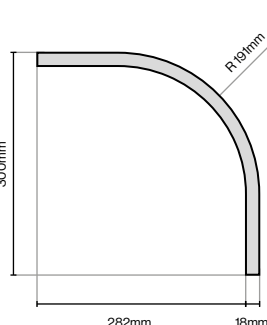
Curved Plain Plinth 300mm (L) x 300mm (W) x 150mm (H)
