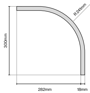
Curved Tangent Pelmet 300mm (L) x 300mm (W) x 150mm (H)
