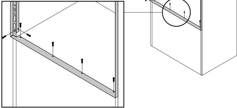
Figure 2 / Lower Heat Deflector Assembly
