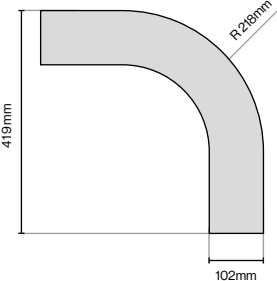
Curved Classic Cornice (Smooth) 419mm (L) x 419mm (W) x 70mm (H)
