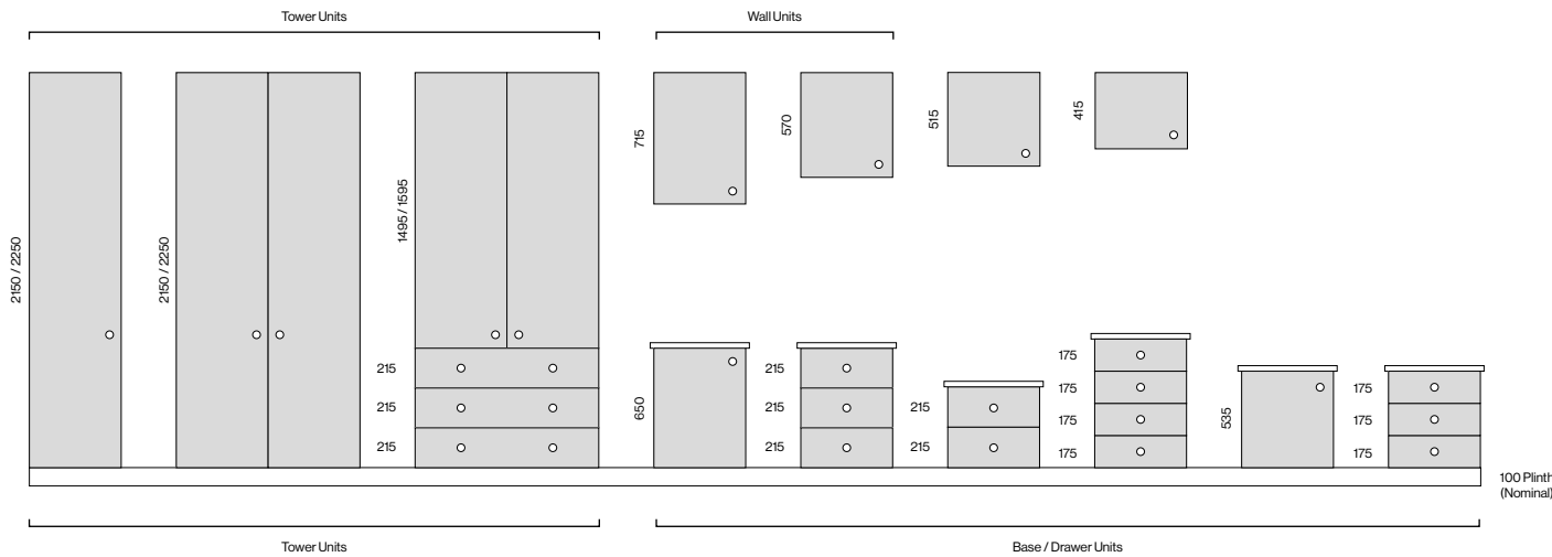
Standard Bedroom / 2150mm / 2250mm / Base and Full Height Unit Door Configurations
