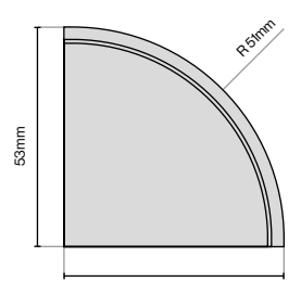
Under Cornice Quadrant (Smooth) 53mm (L) x 53mm (W) x 30mm (H)
