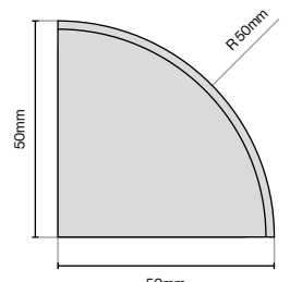
Modern Cornice / Pelmet Quadrant 50mm (L) x 50mm (W) x 30mm (H)
