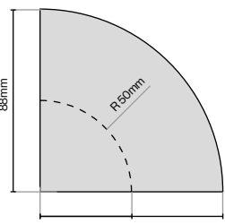
Tangent Cornice Quadrant 88mm (L) x 88mm (W) x 44mm (H)
