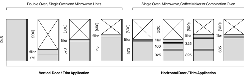
1250mm / Studio Height Unit Door and Appliance Configurations
