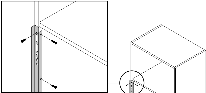
Figure 1 / Side Heat Deflector Assembly
