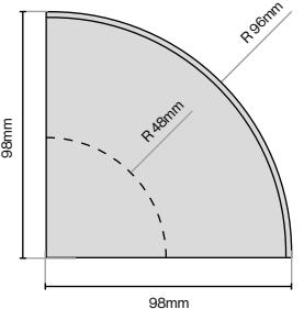
Classic Cornice Quadrant (Smooth) 98mm (L) x 98mm (W) x 70mm (H)
