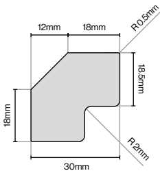
Corner Post 3050mm Lengths
