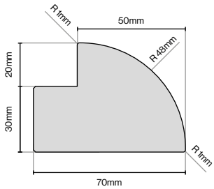
Radius Profile 3050mm Lengths
