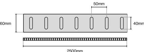
Fluted Rail 2500mm (L) x 18mm (W) x 60mm (H)
