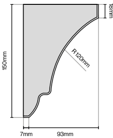
Shelf Bracket 100mm (L) x 18mm (W) x 150mm (H)
