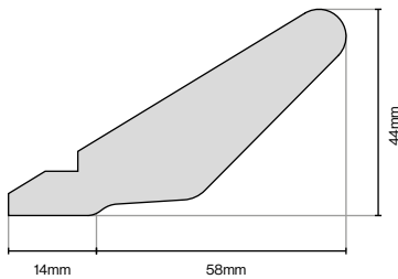
Tangent Cornice 3050mm Lengths
