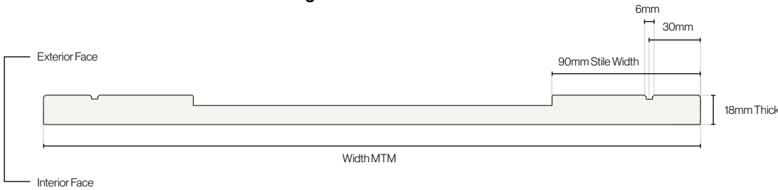
Wellington Door Cross Section
