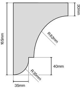
Classic Corbel 125mm (L) x 90mm (W) x 165mm (H)
