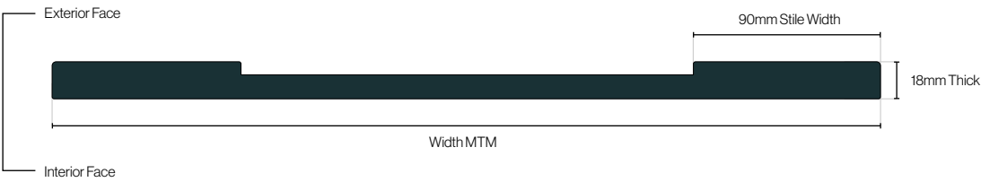
Hartford Door Cross Section
