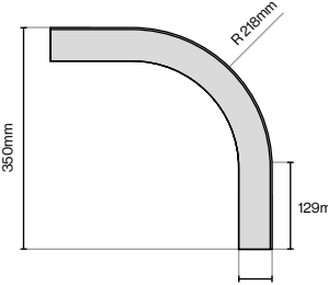
Curved Under Cornice (Smooth) 350mm (L) x 350mm (W) x 30mm (H)
