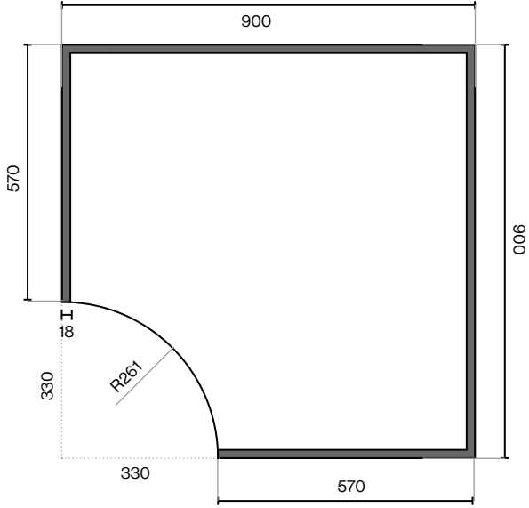
330mm Concave Door 330mm x 330mm Concave Door for 900mm Base Unit
