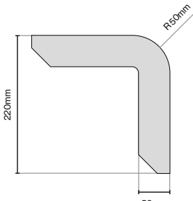
Modern Cornice / Pelmet Quadrant 220mm (L) x 220mm (W) x 30mm (H)
