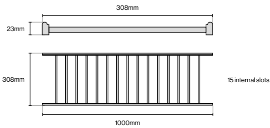
Plate Cot 1000mm (L) x 23mm (W) x 308mm (H)
