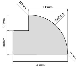
Radius Profile 3050mm Lengths
