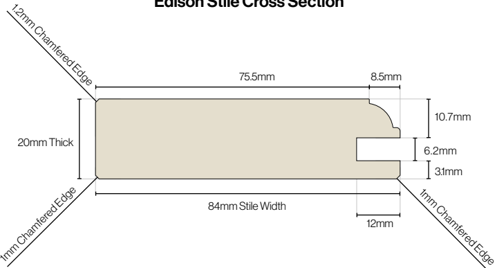
Edison Stile Cross Section
