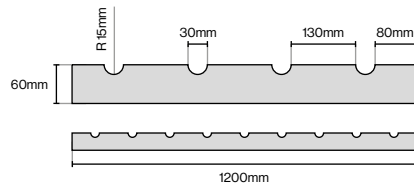
Wine Rack Rail 1200mm (L) x 18mm (W) x 60mm (H)
