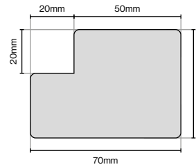
Square Pilaster 3050mm Lengths
