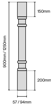
Turned Pilaster (Solid Timber) 900mm (H) x 94mm (W) 900mm (H) x 57mm (W) 1250mm (H) x 57mm (W)
