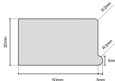
Under Cornice (Smooth) 3050mm Lengths
