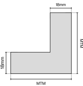
MTM Corner Post 715mm (150 x 150mm Max)
