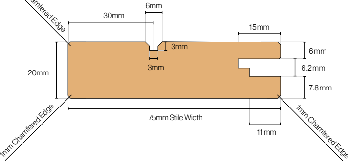
Campbell Oak Stile Cross Section
