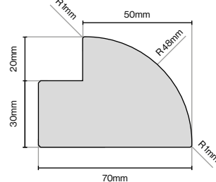
Radius Profile 3050mm Lengths
