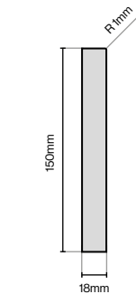
Plain Plinth 3050mm Lengths
