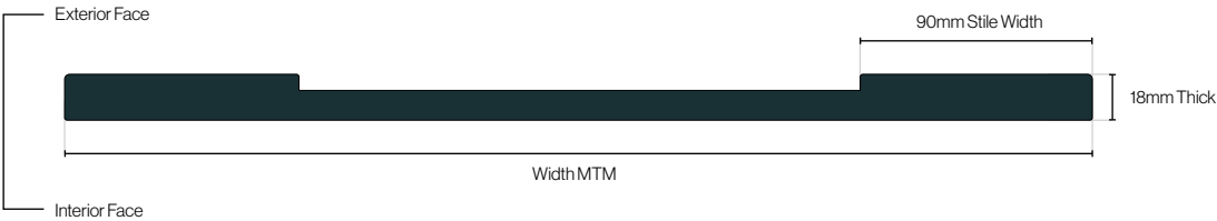
Hartford Door Cross Section
