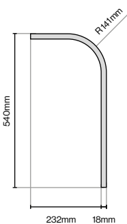
Curved Plain Plinth 540mm (L) x 250mm (W) x 150mm (H)
