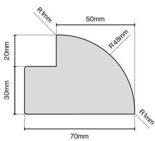
Radius Profile 3050mm Lengths
