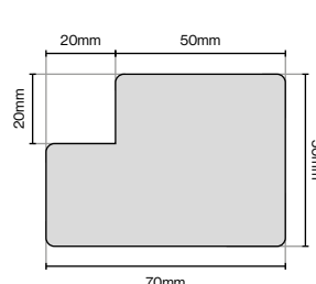
Square Pilaster 3050mm Lengths
