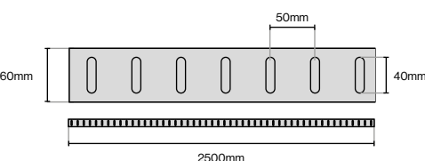
Fluted Rail 2500mm (L) x 18mm (W) x 60mm (H)
