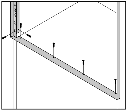
Figure 2 / Lower Heat Deflector Assembly
