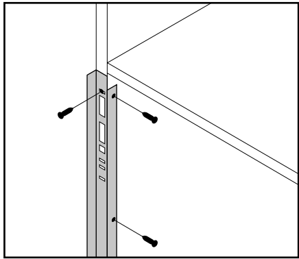
Figure 1 / Side Heat Deflector Assembly
