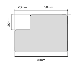
Square Pilaster 3050mm Lengths
