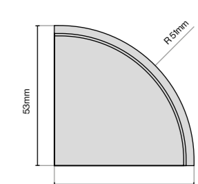
Under Cornice Quadrant (Smooth) 53mm (L) x 53mm (W) x 30mm (H)
