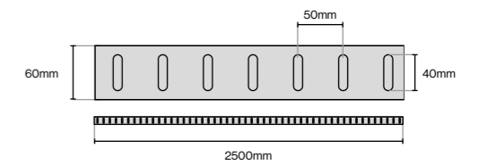
Fluted Rail 2500mm Lengths
