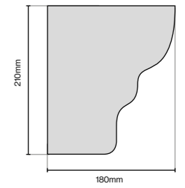
Shelf Bracket 180mm (L) x 37mm (W) 210mm (H)
