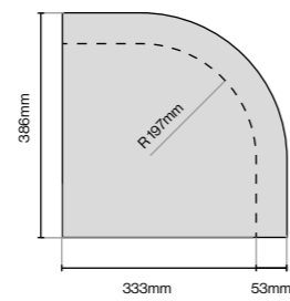
Curved Classic Cornice 386mm (L) x 333mm (W) x 53mm (H)
