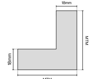
MTM Corner Post 715mm (150 x 150mm Max)
