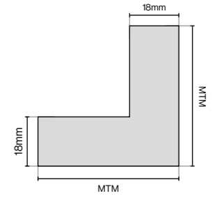
MTM Corner Post 715mm (150 x 150mm Max)
