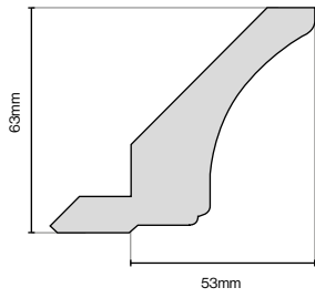
Classic Cornice 3050mm Lengths
