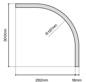
Curved Torus Plinth 300mm (L) x 300mm (W) x 150mm (H)
