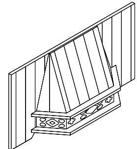
Traditional Canopy 1000mm (W) x 193mm (D) x 525mm (H) Supplied with fretwork and T&G detail as standard. Fretwork detail can be removed on request.
