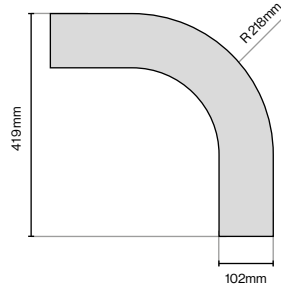
Curved Classic Cornice (Smooth) 419mm (L) x 419mm (W) x 70mm (H)
