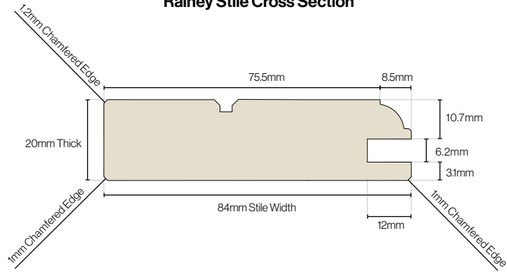
Rainey Stile Cross Section
