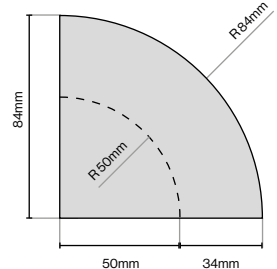
Classic Cornice Quadrant 84mm (L) x 84mm (W) x 63mm (H)
