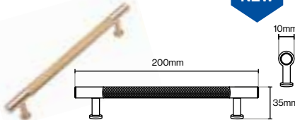
Fender Knurled 'D' Handle
