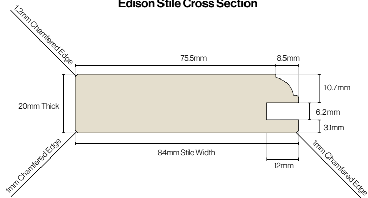
Edison Stile Cross Section
