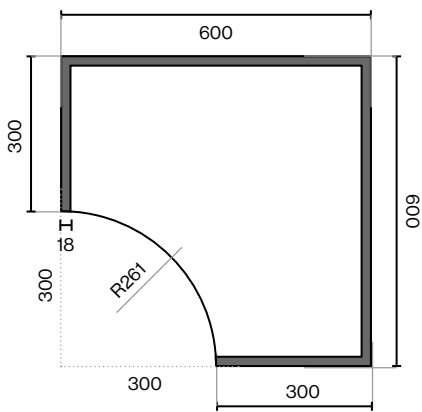
300mm Concave Door 300mm x 300mm Concave Door for 600mm Wall Unit
