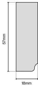
Tangent Light Pelmet 3050mm Lengths
