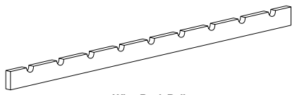
Wine Rack Rail 1200mm (L) x 18mm (W) x 60mm (H)
