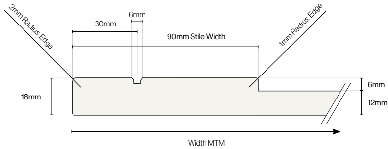
Wellington Stile Cross Section
