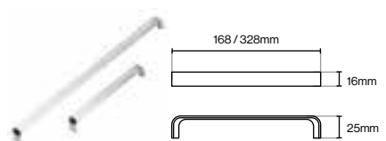
Camden 'D' Handle
