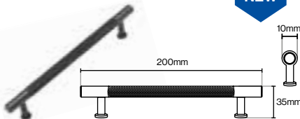
Fender Knurled 'D' Handle
