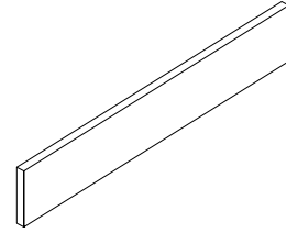
Plain Plinth 18mm (W) x 150mm (H) 2400mm Lengths
