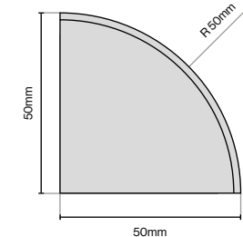
Modern Cornice / Pelmet Quadrant 50mm (L) x 50mm (W) x 30mm (H)
