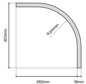
Curved Torus Plinth 300mm (L) x 300mm (W) x 150mm (H)
