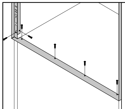
Figure 2 / Lower Heat Deflector Assembly
