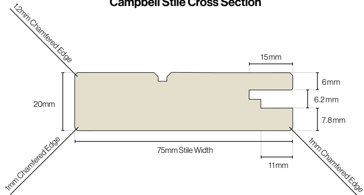
Campbell Stile Cross Section
