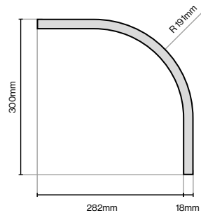
Curved Plain Plinth 300mm (L) x 300mm (W) x 150mm (H)
