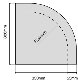
Curved Classic Cornice 386mm (L) x 336mm (W) x 63mm (H)
