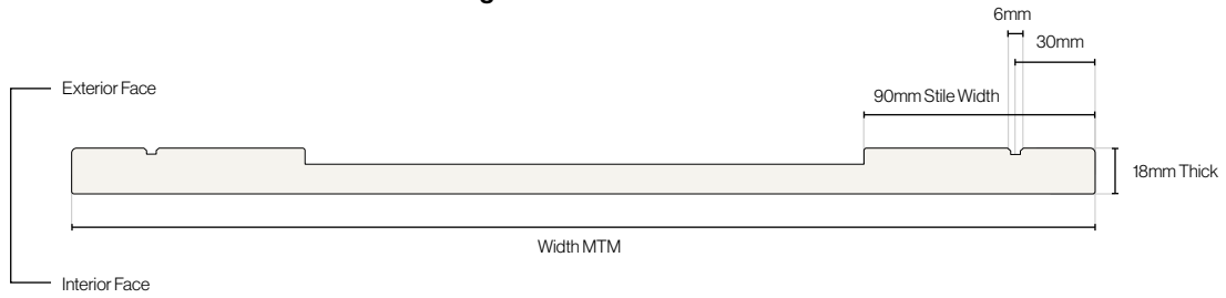
Wellington Door Cross Section
