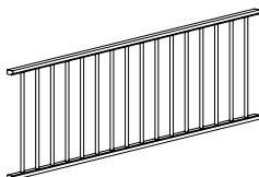
Plate Cot (Pair) / 1000mm (L) x 23mm (W) x 308mm (H)
