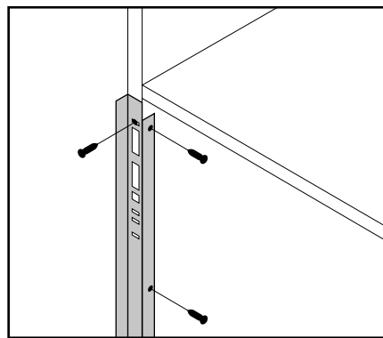
Figure 1 / Side Heat Deflector Assembly
