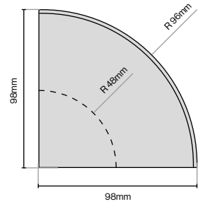
Classic Cornice Quadrant (Smooth) 98mm (L) x 98mm (W) x 70mm (H)
