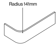
Curved Plain Plinth 540mm (L) x 232mm (W) x 150mm (H)
