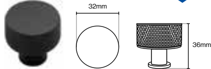
Fender Knurled Knob
