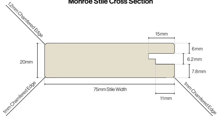
Monroe Stile Cross Section
