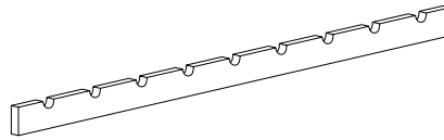
Wine Rack Rail 1200mm (L) x 18mm (W) x 60mm (H)
