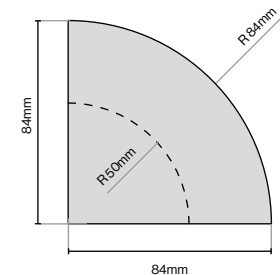
Classic Cornice Quadrant (Grained) 84mm (L) x 84mm (W) x 63mm (H)
