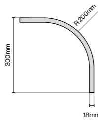
Curved Torus Plinth (Smooth)
