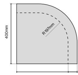
Curved Tangent Cornice 400mm (L) x 400mm (W) x 44mm (H)
