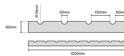
Wine Rack Rail
