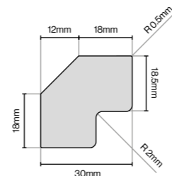
Corner Post
