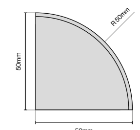
Modern Cornice / Pelmet Quadrant 50mm (L) x 50mm (W) x 30mm (H)
