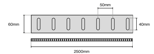
Fluted Rail
