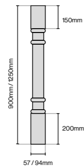
Turned Pilaster (Solid Timber)
