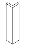
External Corner Post 685 x 46 x 46mm
