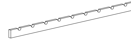
Wine Rack Rail 1200mm (L) x 18mm (W) x 60mm (H)
