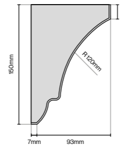
Shelf Bracket
