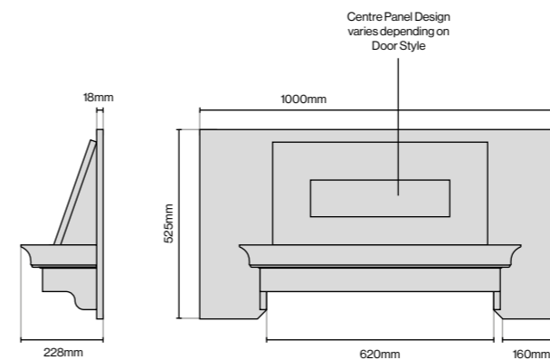
Modern Canopy
