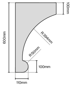
French Mantle Corbel
