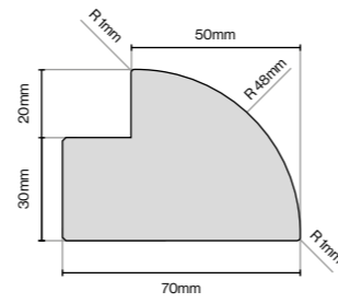
Radius Profile
