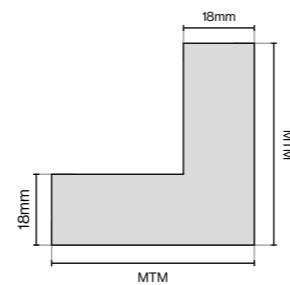
MTM Corner Post
