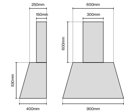
Chimney Canopy
