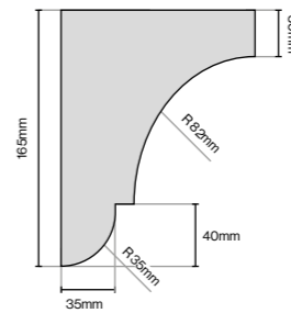
Classic Corbel
