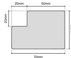
Square Pilaster
