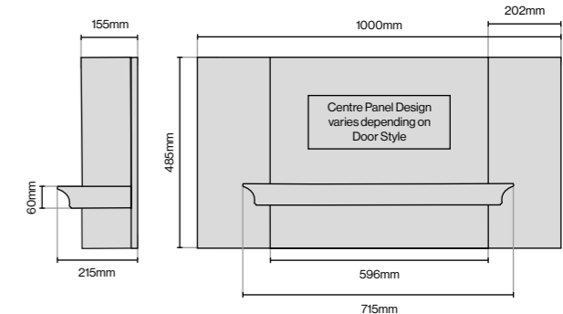
Classic Canopy
