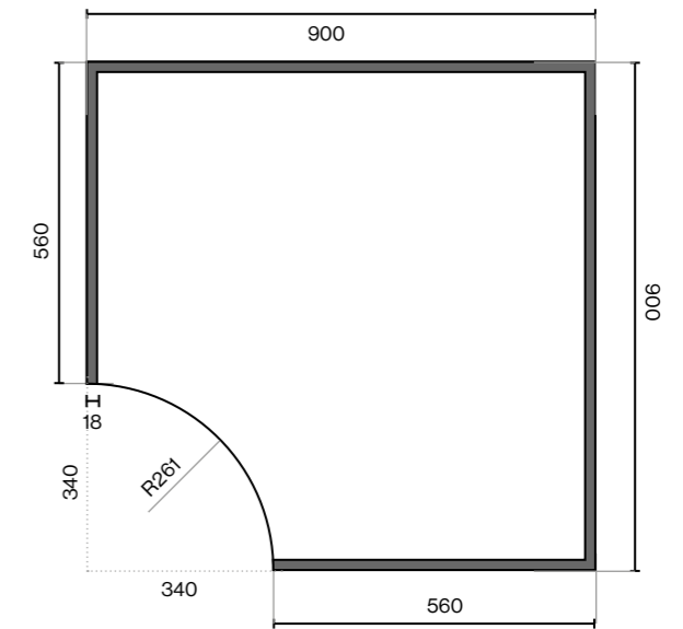
340mm Concave Door 340mm x 340mm Concave Door for 900mm Base Unit
